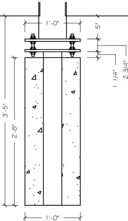
A DETAIL-BASE PLATE 3" = 1'-0"
