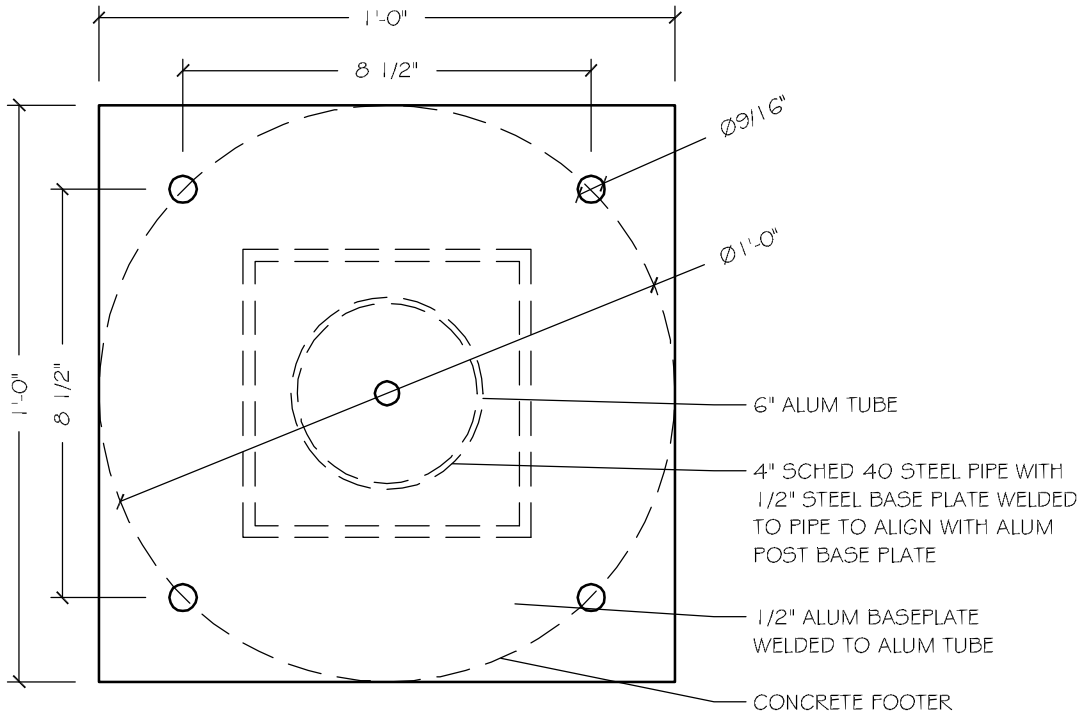
A DETAIL-BASE PLATE 3" = 1'-0"
