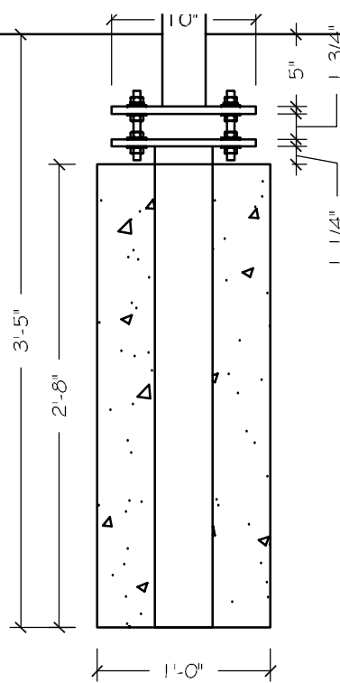
A DETAIL-BASE PLATE 3" = 1'-0"
